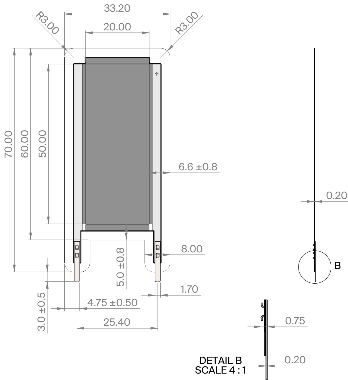
Figure 10. Mechanical dimensions and tolerances of Epishine's modules on the example of an OC15_20x50_1_10 module.
